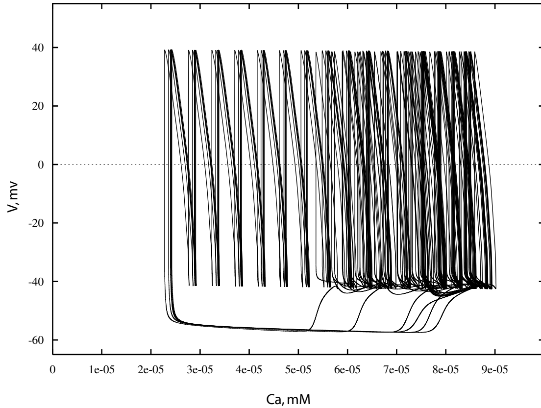
Projection on to (Ca, V) plane
