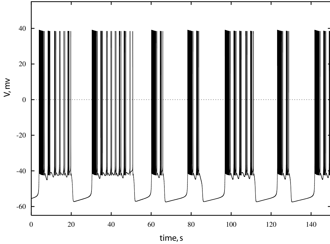
Time course of membrane potential
